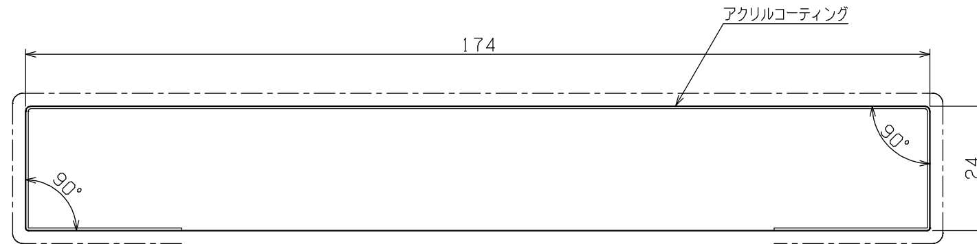
断面形状詳細 (SCALE 1/1)
