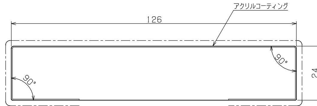
断面形状詳細 (SCALE 1/1)
