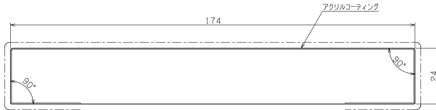
断面形状詳細 (SCALE 1/1)
