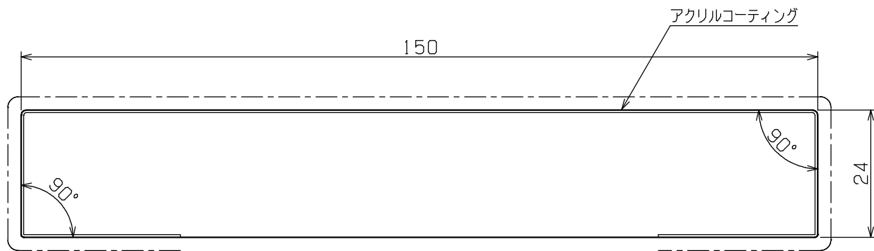
断面形状詳細 (SCALE 1/1)
