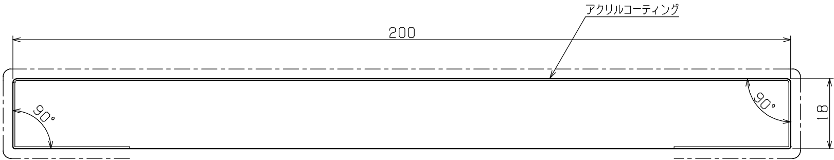
断面形状詳細 (SCALE 1/1)
