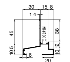
HKA-30-L27 (出幅30mm)
